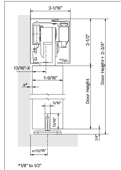
Vertical section
